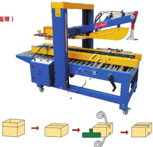
下左右驱动折盖封箱机 Bottom left-right driven flap case-sealing machine
