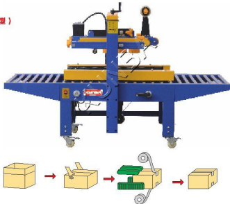
下左右驱动折盖封箱机 Bottom left-right driven flap case-sealing machine
