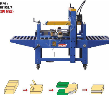
上下驱动侧封箱机 Top-bottom driven side carton sealer
