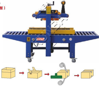
上左右驱动封箱机 Top-left-right-driven carton sealer
